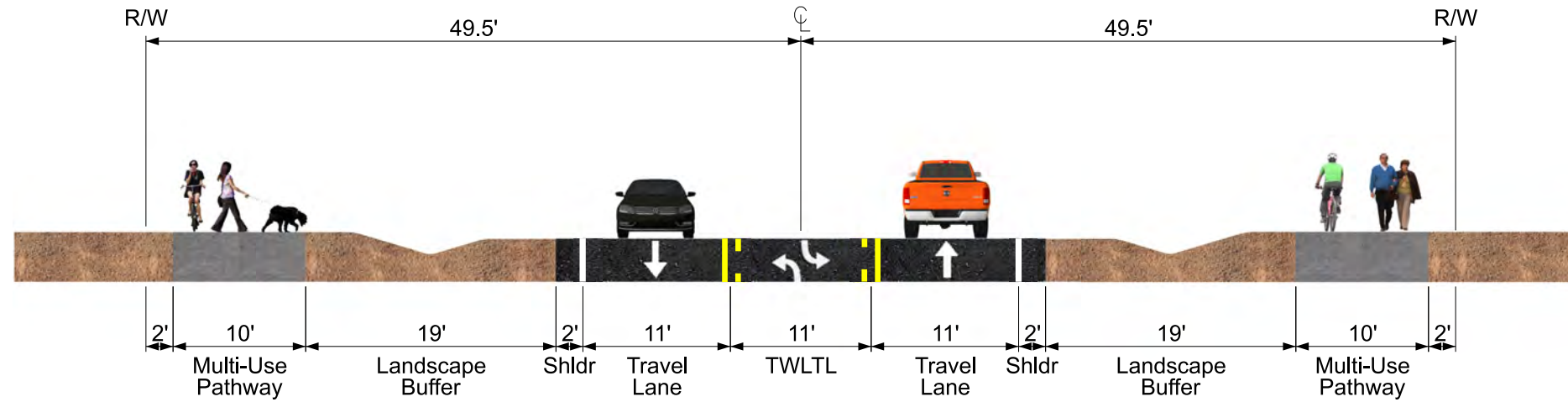
3 Lane Alternative (One Lane In Each Direction With A Center Turn Lane)
