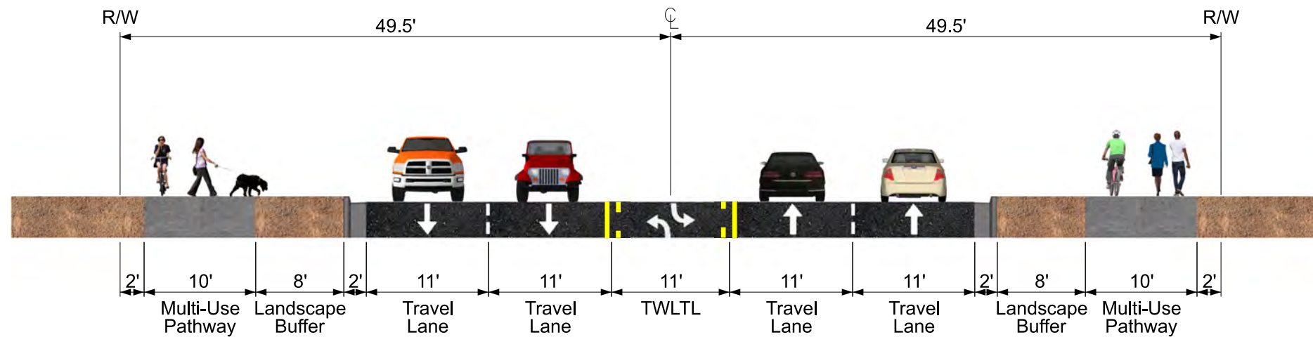
5 Lane Alternative (Two Lanes In Each Direction With A Center Turn Lane)
