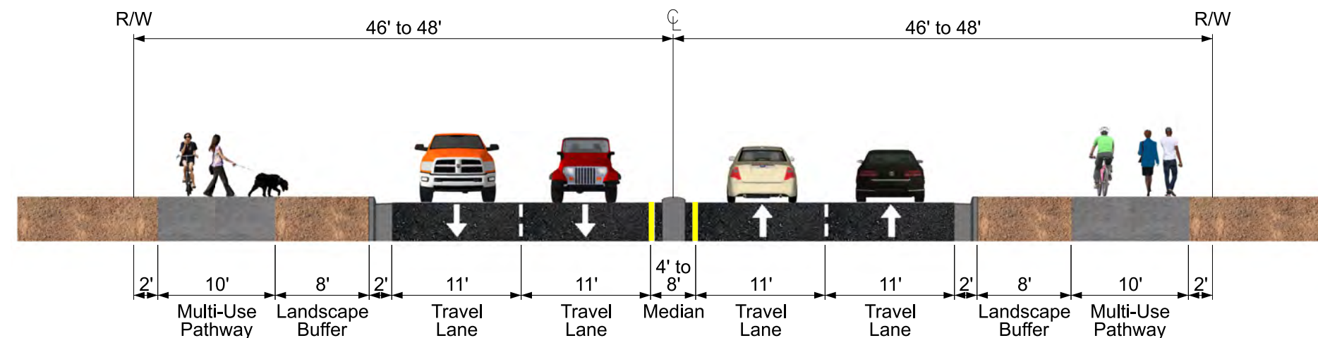
4 Lane Alternative (Two Lanes In Each Direction With A Center Median And Roundabouts At Key Intersections)
