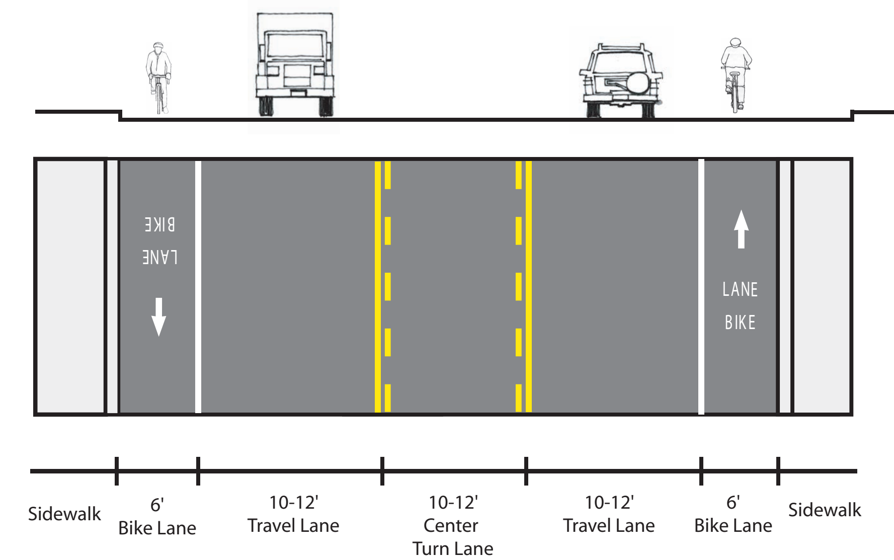
3-Lanes (No Parking) (Emerald)
