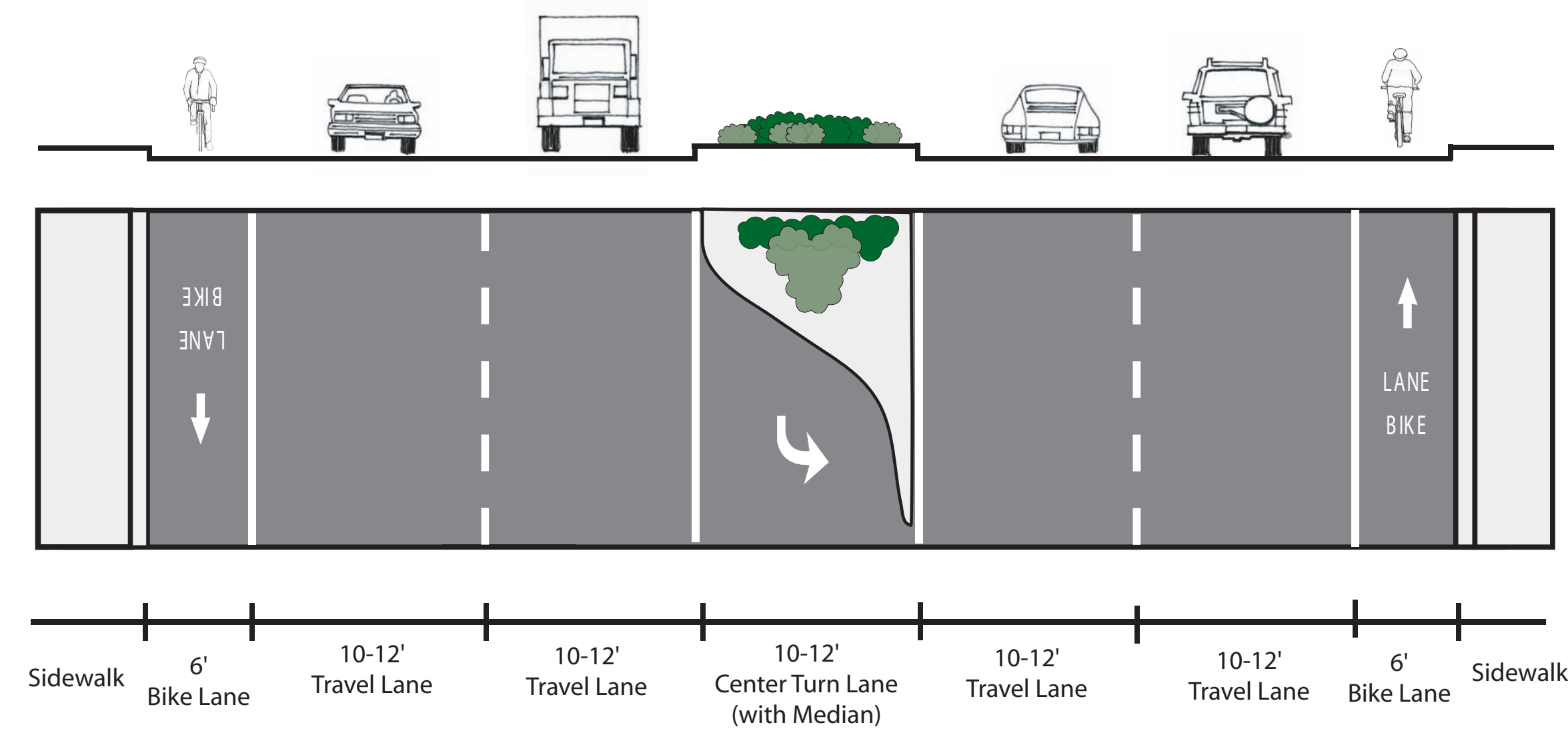
5-Lanes (No Parking) (Overland in Meridian/Curtis)
