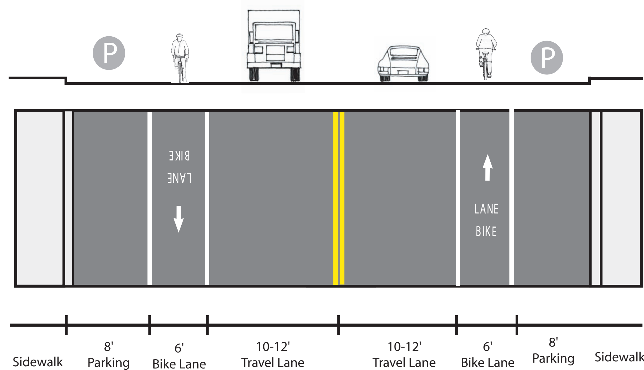
Two Lanes with Parking Two Sides (Linda Vista)
