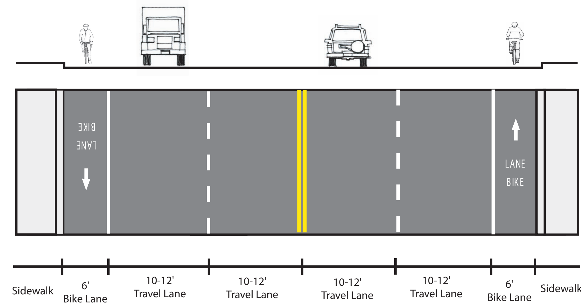
4-Lanes (No Parking) (Victory, McMillan)
