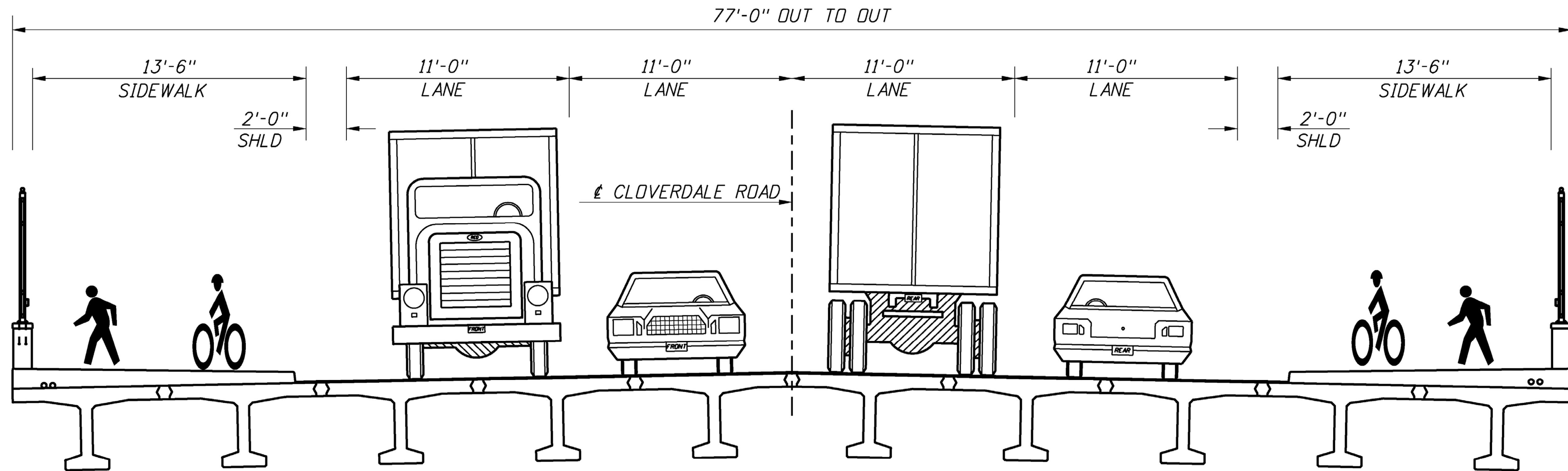
10 - 49" DECK BULB TEE GIRDERS TYPICAL SECTION
