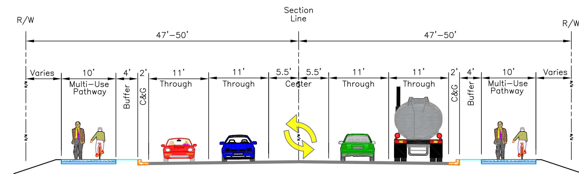
Lake Hazel Road - East & West Corridor N.T.S.
