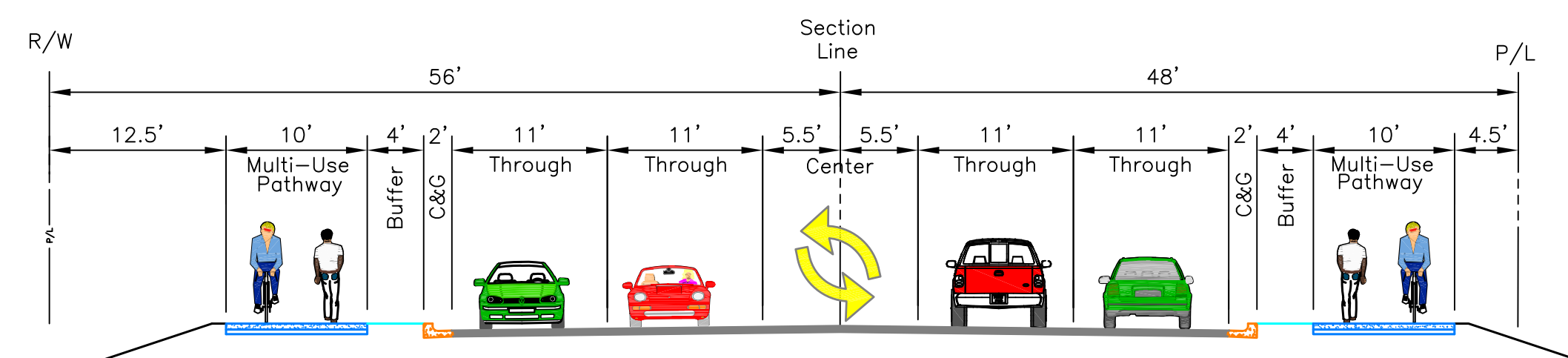
Eagle Road - North Corridor N.T.S.
