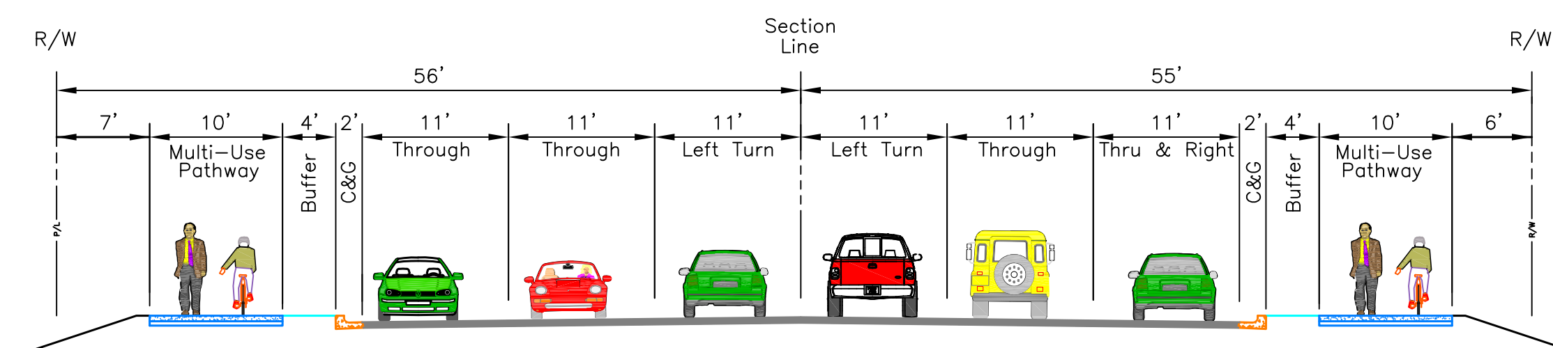
Lake Hazel Road - West Leg Of Intersection N.T.S.
