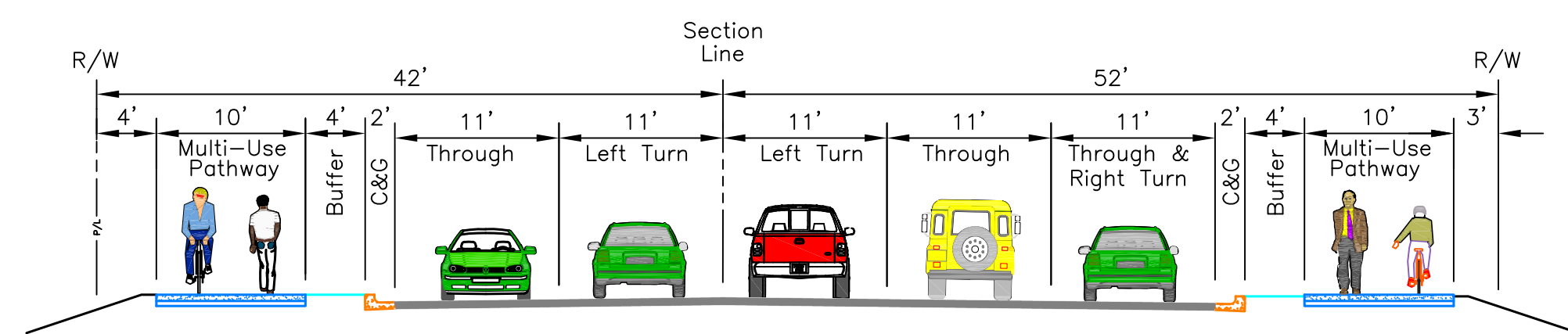
Eagle Road - South Leg Of Intersection N.T.S.
