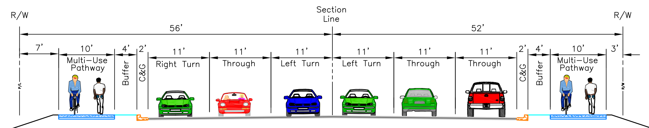
Eagle Road - North Leg Of Intersection N.T.S.
