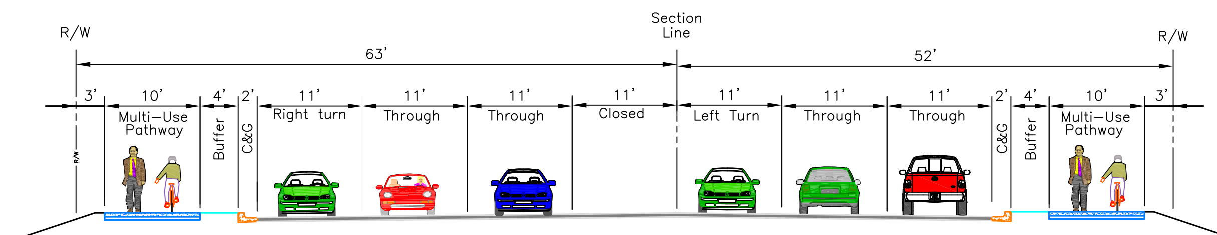
Lake Hazel Road - East Leg Of Intersection N.T.S.
