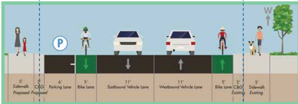
Option 2: Bike lanes, south side sidewalk
