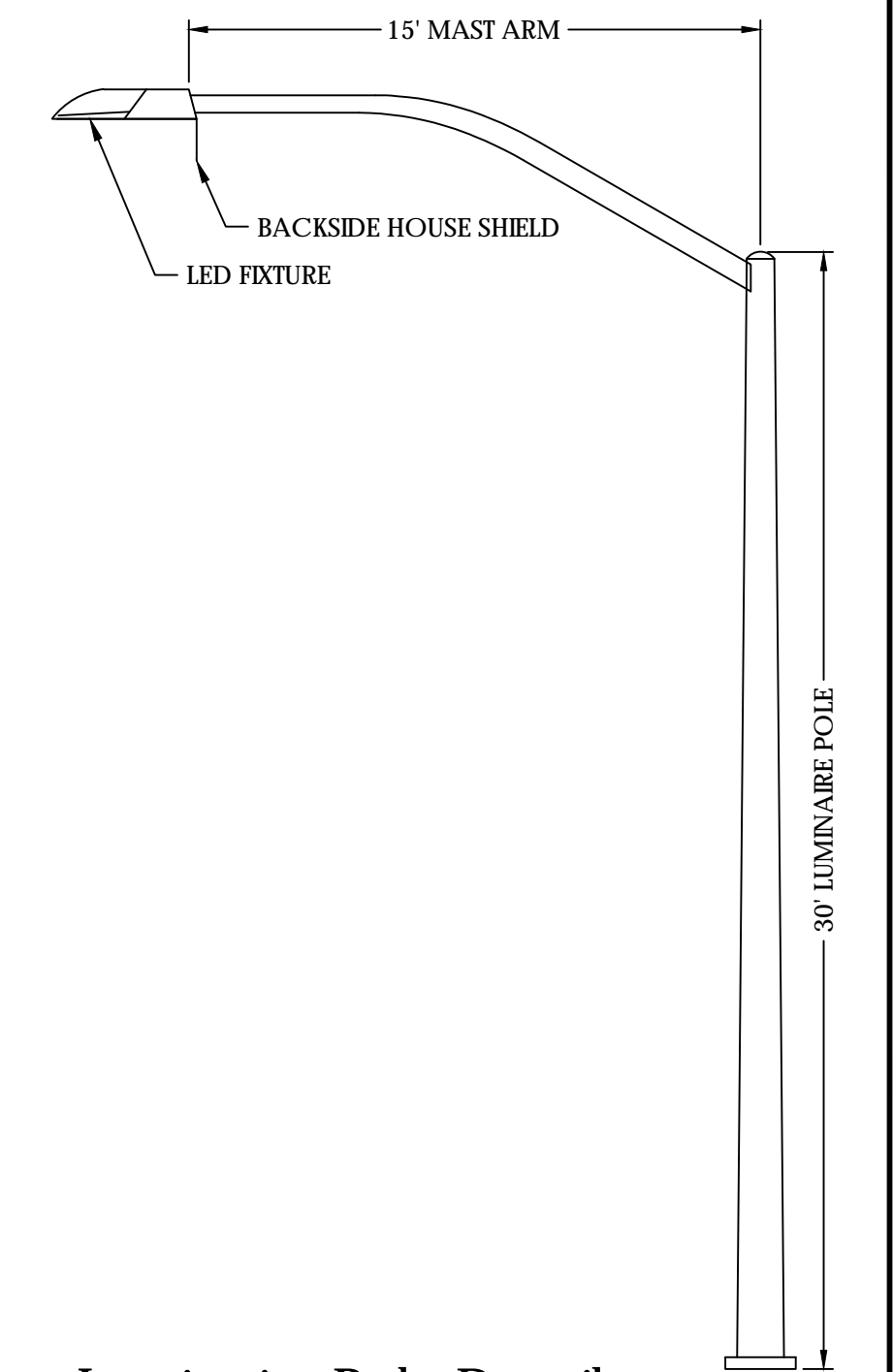
Luminaire Pole Detail
