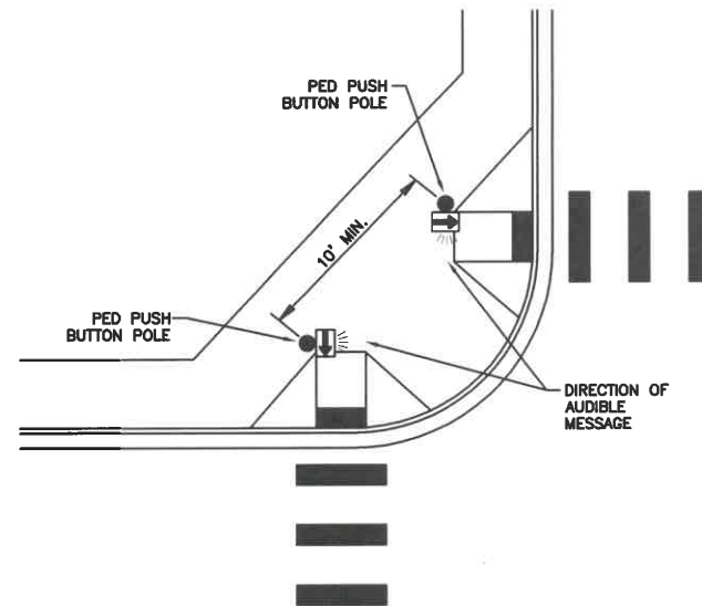
'IDEAL' PED PUSH BUTTON PLACEMENT
