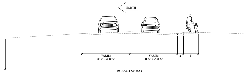
ALPINE STREET SIDEWALK CONCEPT
