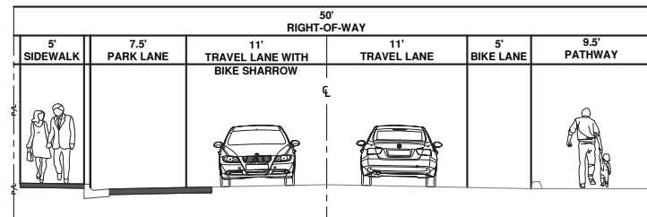
N ROOSEVELT STREET TYPICAL SECTION (NORTH OF ALPINE STREET)
