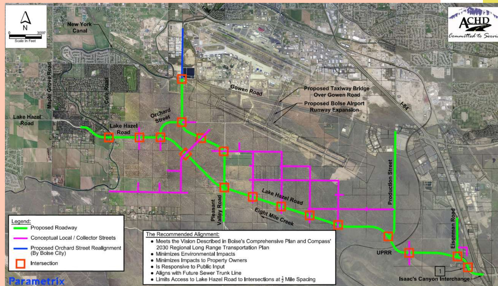
Figure 8-2. Recommended Alignments
