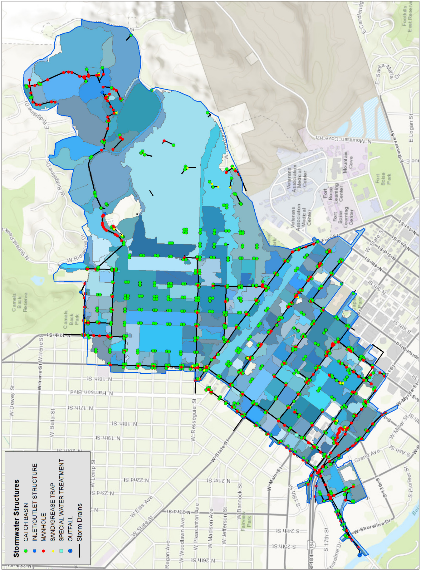
■ Figure 11. Americana Subwatershed Subareas (Grouped) with Storm Drains and Stormwater Infrastructure
