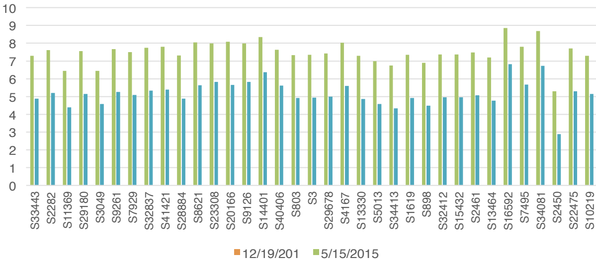
Figure 20. E.coli load (mil. Col.) from two modeled (PCSWMM) WQ storms
